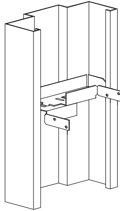
ADJUSTABLE ANCHOR
