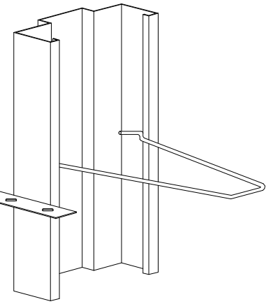
MASONRY WIRE ANCHOR
