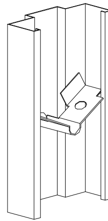
EXISTING MASONRY ANCHOR
