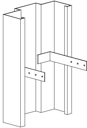
STRAP ANCHOR
